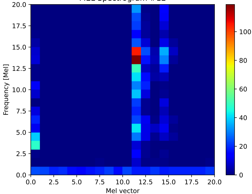
MEL Spectrogram #12
